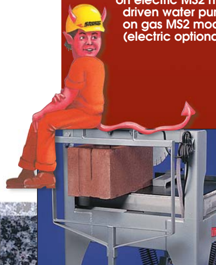
Open back design permits rip cutting of large blocks and masonry materials. No need to turn block multiple times.
