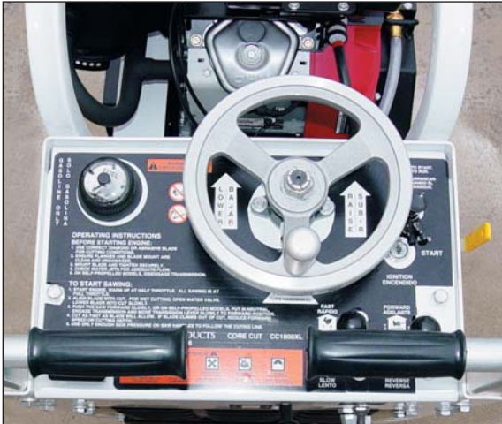
CC1800XL Control Panel (remote throttle, choke and ignition switch are only available on 20 HP models)
